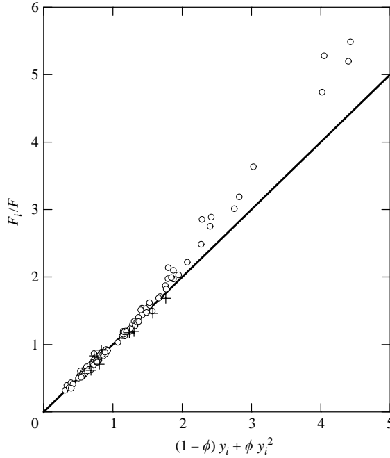
FIGURE 8. Individual drag force F_i divided by the drag force F of a monodisperse system at the same \phi , as a function of (1-\phi)y_i + \phi y_i^2 . The circles represent the simulation data from table 2, the plus symbols the simulation results from Koo & Sangani (2002); the solid line is the theoretical prediction given by (32). Note that assumption F_i = F , which is used in many numerical models, differs by up to a factor of 5 with the simulation data.
